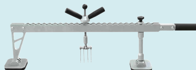
Double action levelling bar ref. 053564
