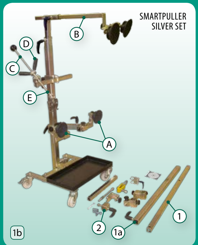
The Figure 1 and 1b. The lower rubber pads (A) of SmartPuller have been adjusted to the proper width and height, after which it has been pushed to the strong point near the area to be pulled. The straightening support (B) has also been set to the roof structure of the car in the height and width direction. After this, the pulling screw (C) has been adjusted to the place that is to be pulled. The actual pulling is done with the crank handle (D). A grapple such as welding wire for pulling, pulling gripper or adhesive cup holder can be attached to the holder on the end of the screw (E), based on the kind of target area to be pulled.
